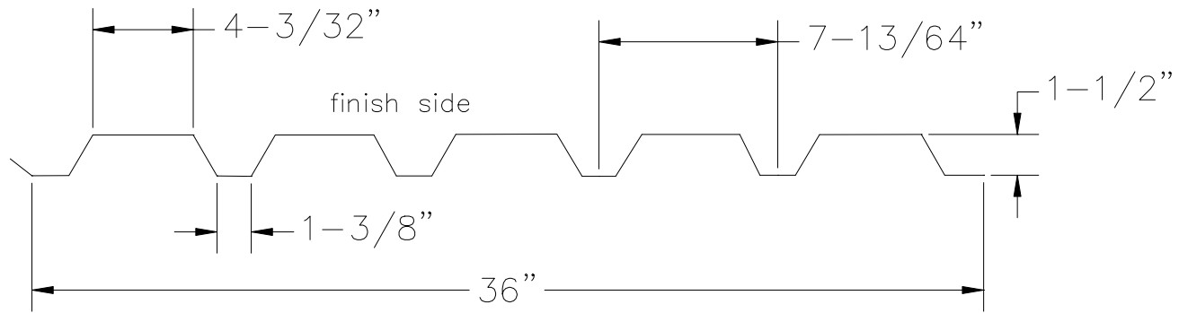
Reverse Box Rib (Roof or Wall Applications Only)
