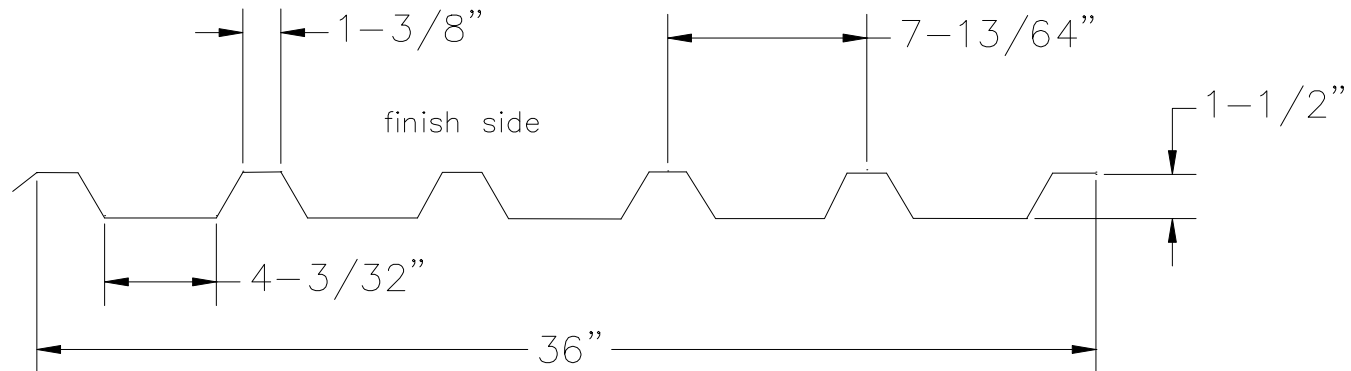
BOX RIB PROFILE
