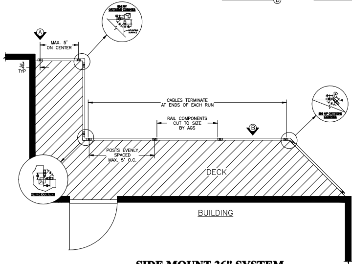
1 SIDE MOUNT 36" SYSTEM WITH STOCK ROUND TOP RAIL COMPONENTS CONTACT AGS FOR CUSTOMIZATION OPTIONS 888-842-9492 OR info@agsstainless.com
