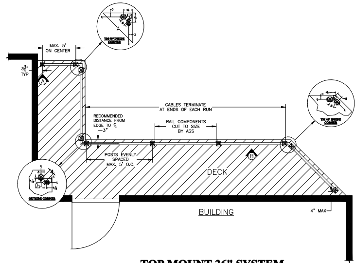
2 TOP MOUNT 36" SYSTEM WITH STOCK ROUND TOP RAIL COMPONENTS CONTACT AGS FOR CUSTOMIZATION OPTIONS 888-842-9492 OR info@agsstainless.com
