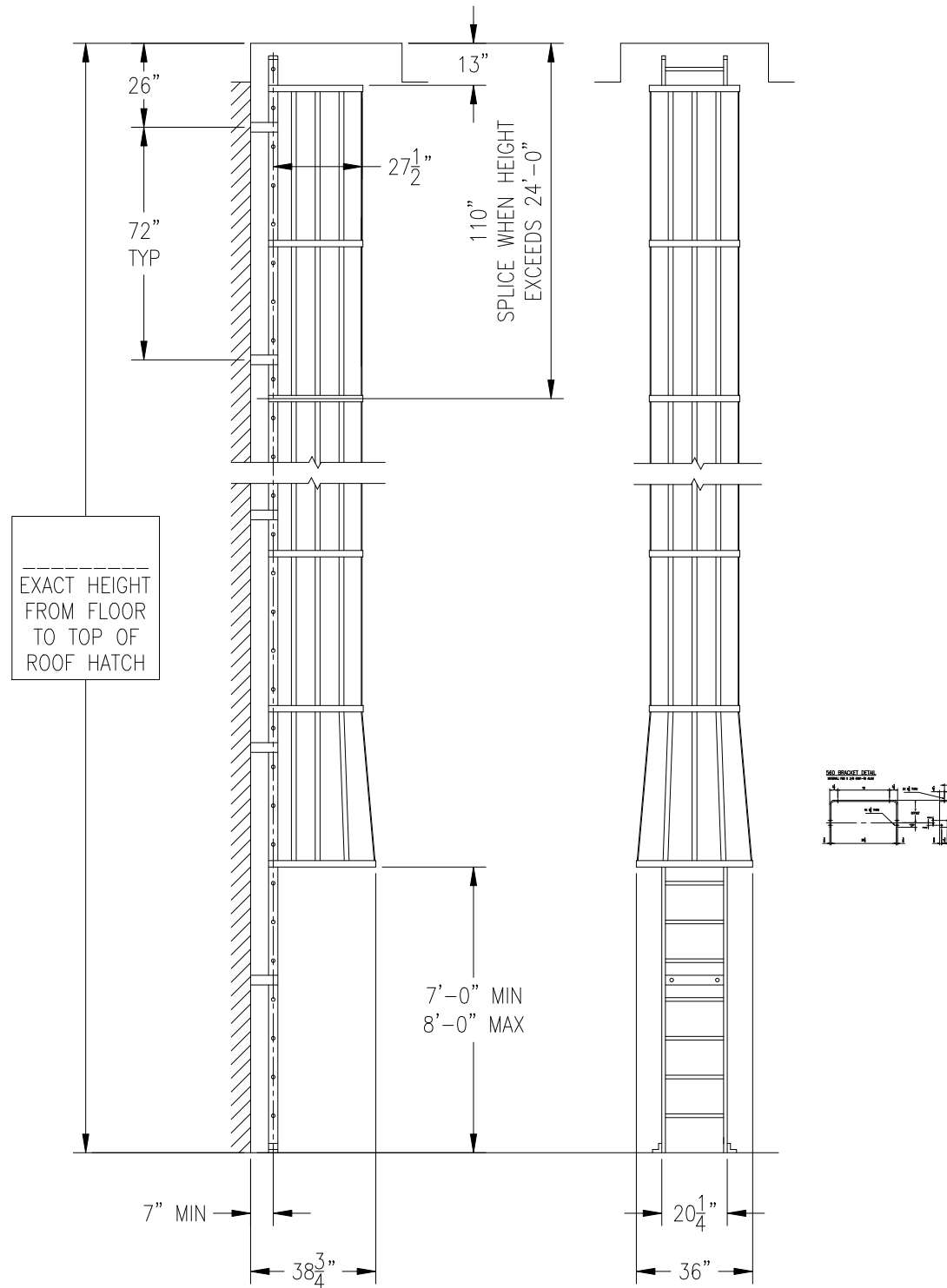
MODEL 560-C CAGED LADDER, ROOF HATCH ACCESS
