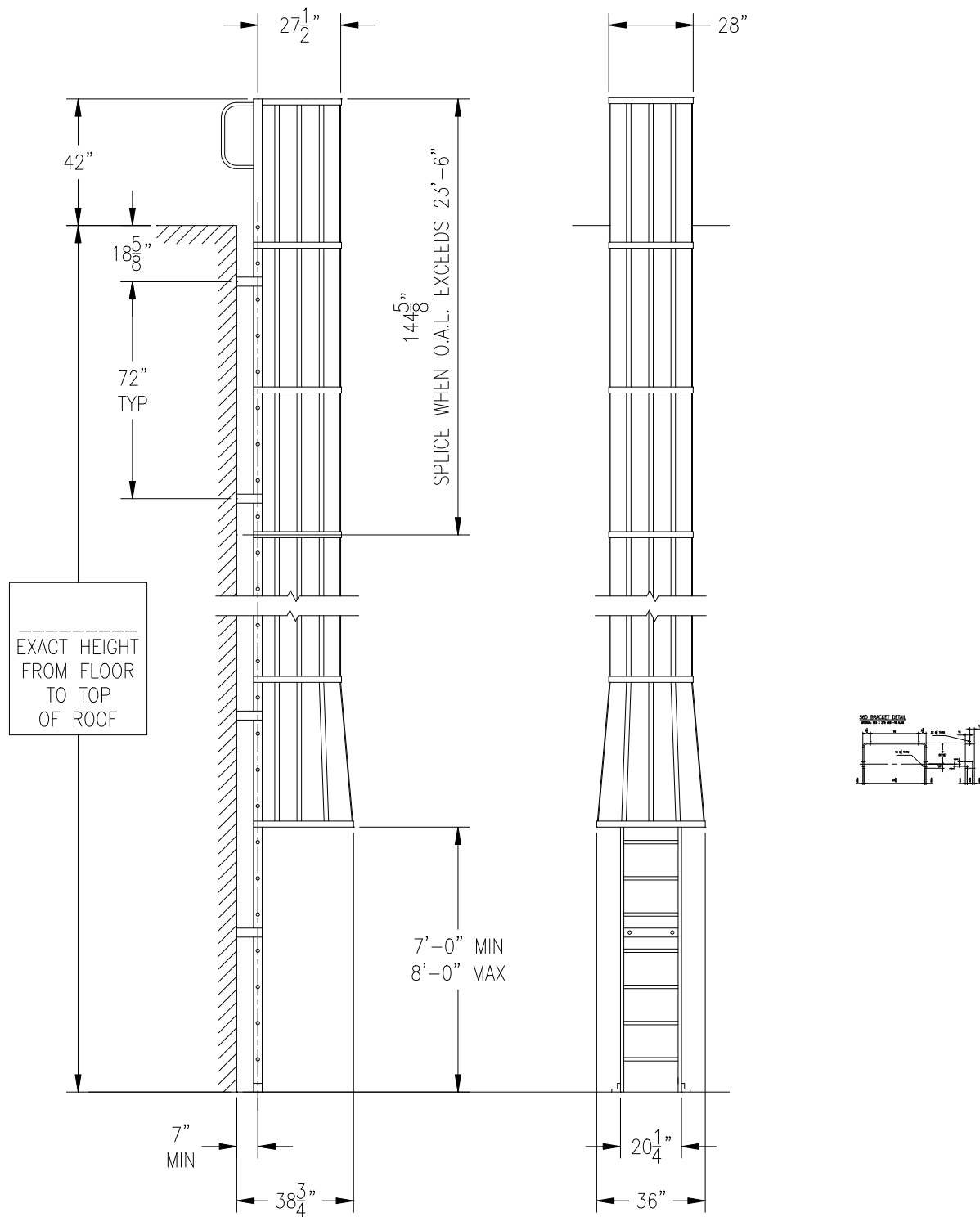
MODEL 561-C CAGED LADDER, HANDRAILS OVER ROOF
