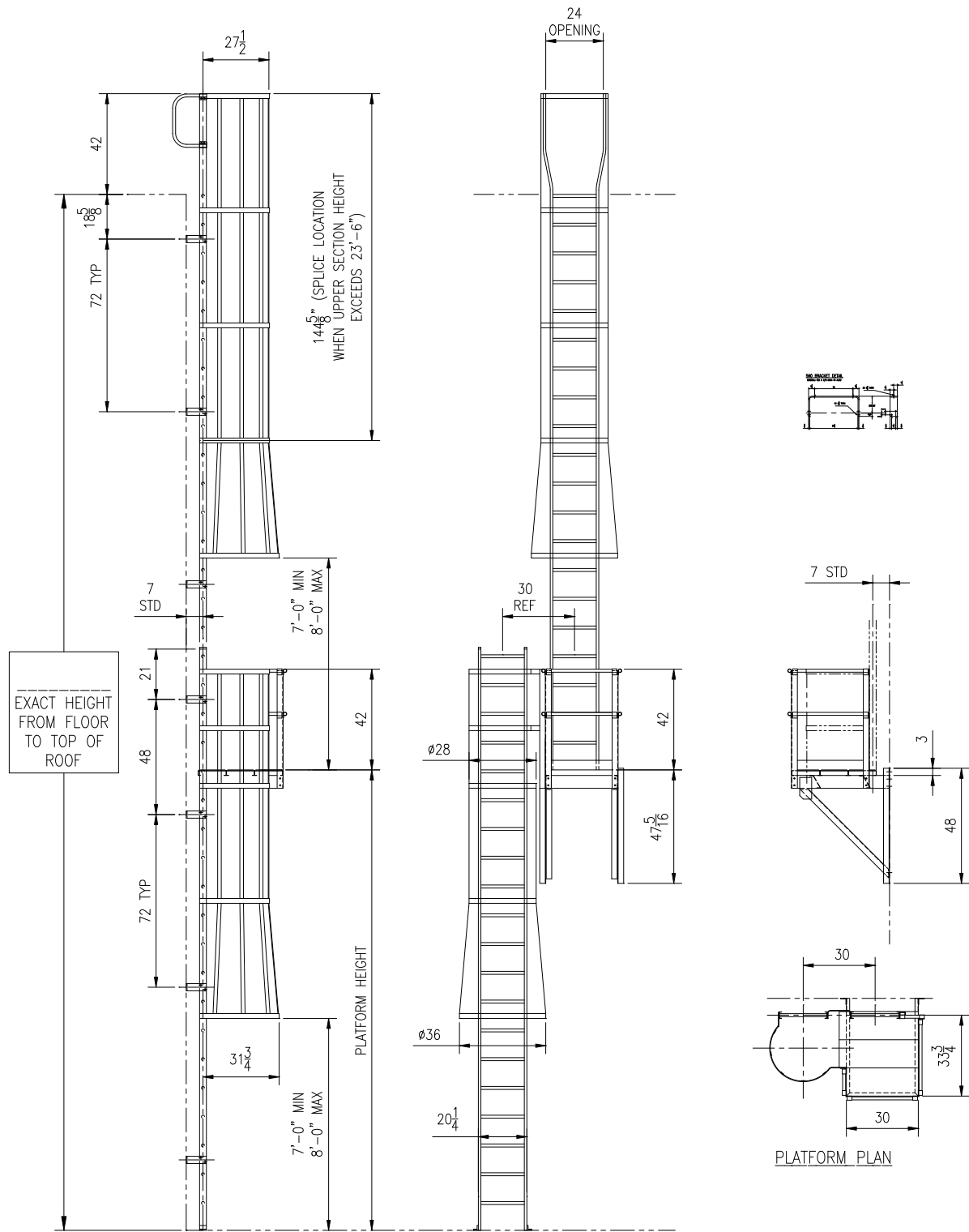
MODEL 561C FIXED WALL LADDER, HANDRAILS OVER ROOF INTERMEDIATE PLATFORM
