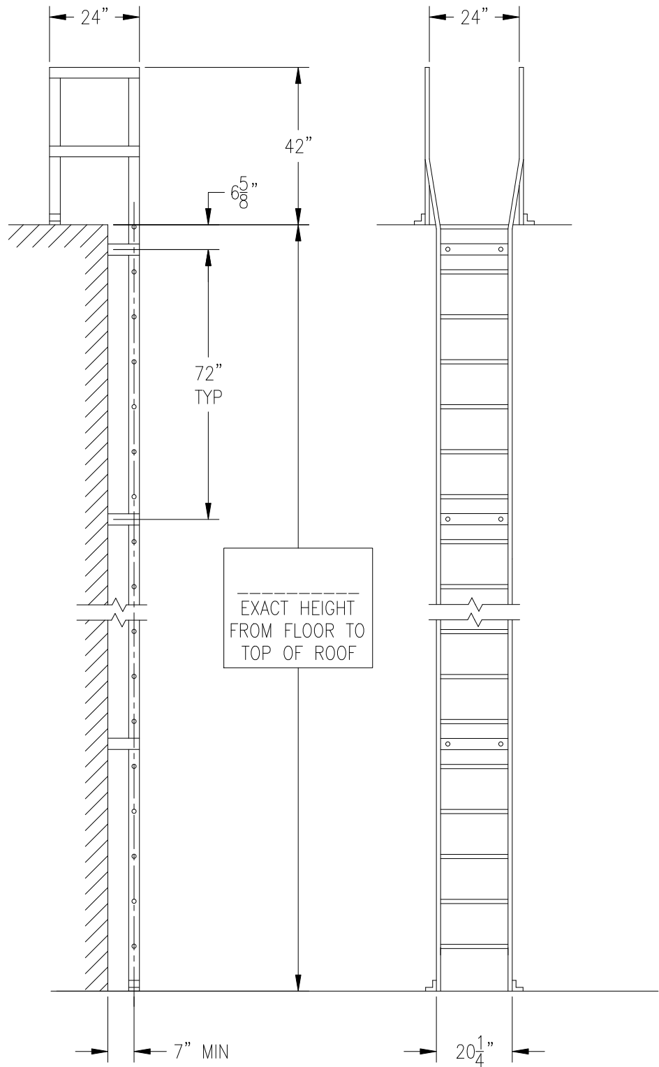
MODEL 562 LADDER, ROOF RETURN
