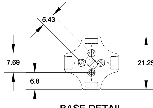
BASE DETAIL
