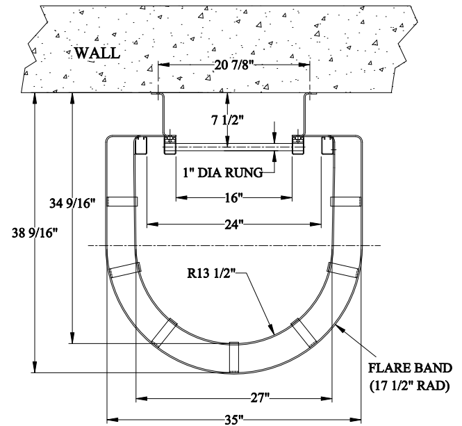
TOP VIEW SUPER LADDER CAGE DETAIL
