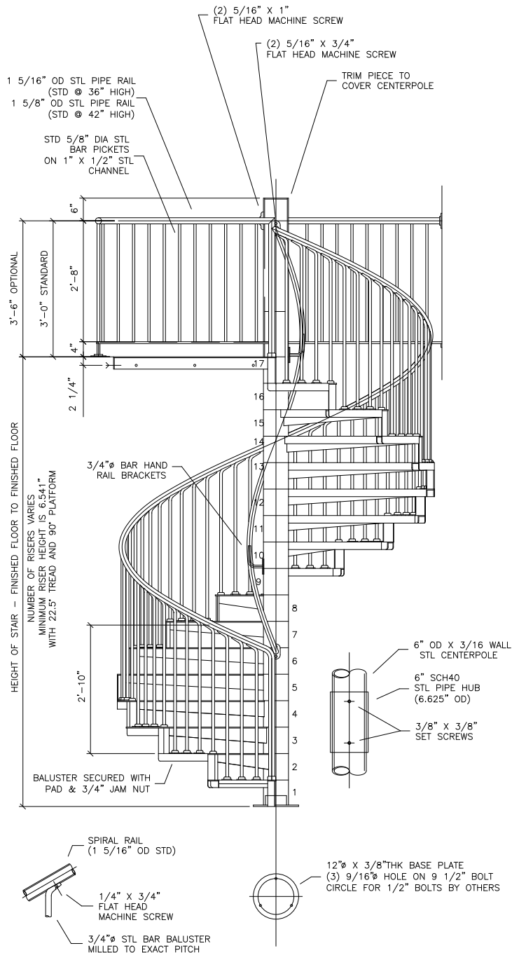
TYPICAL ELEVATION
