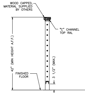
TYPICAL SECTION
