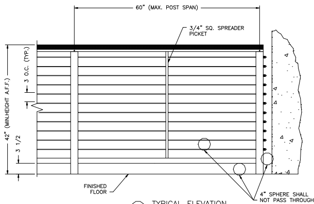
TYPICAL ELEVATION
