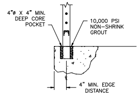
CORE MOUNT
