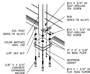
SURFACE MOUNTING DETAIL
