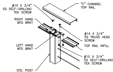
TYP. TOP RAIL CONNECTION
