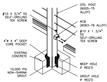
POST ONLY CORE POCKET DETAIL
