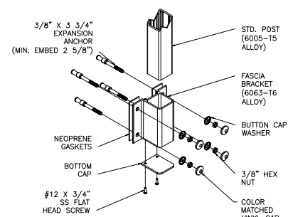
FASCIA MOUNTING DETAIL
