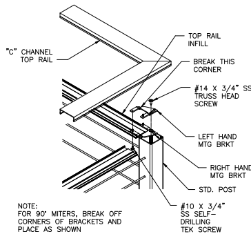
TYP. CORNER CONNECTION
