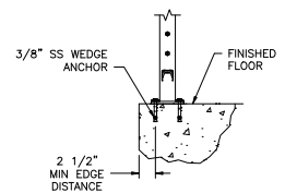
SURFACE MOUNT
