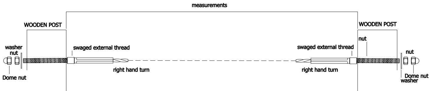
ASSEMBLY 2
