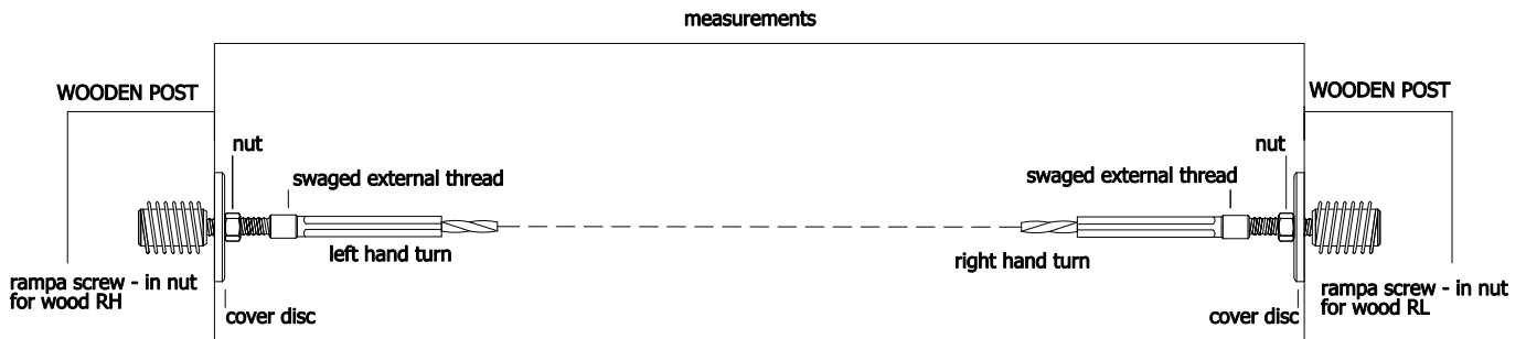
ASSEMBLY 1
