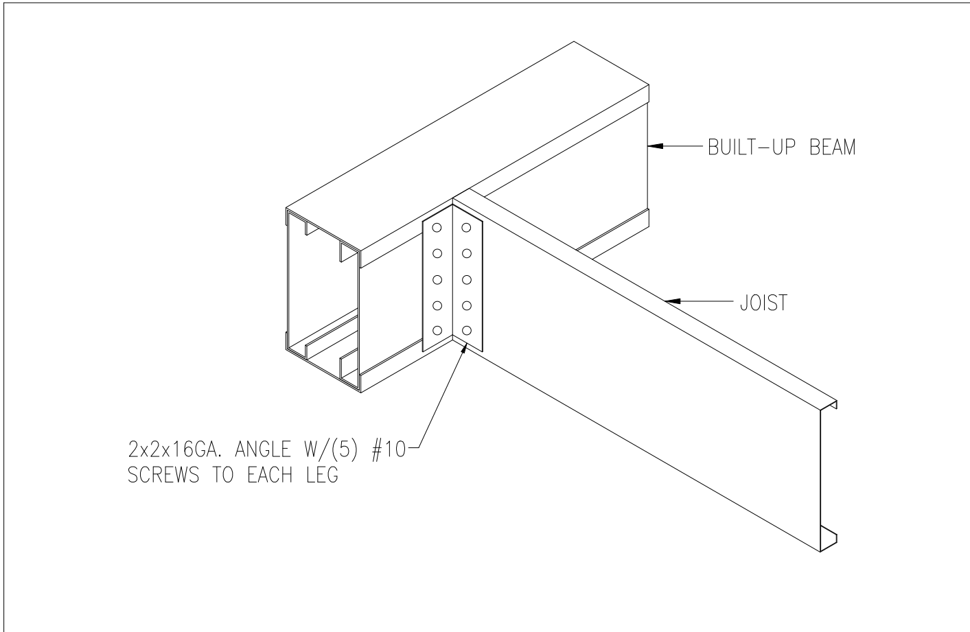
⊖ FLOOR JOIST TO BUILT-UP BEAM N.T.S.
