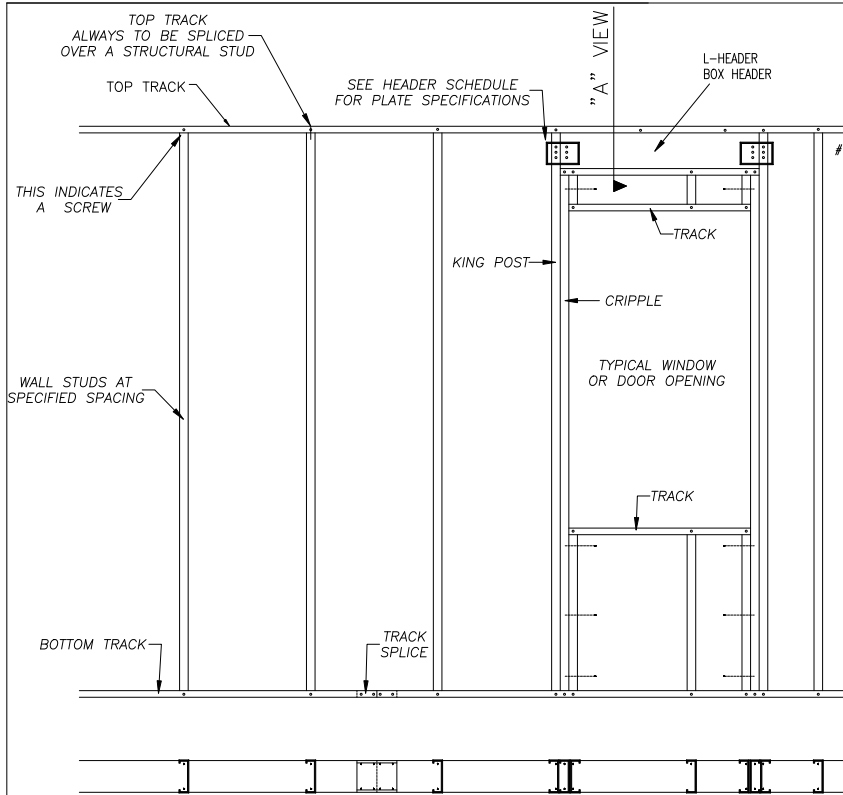
⊖ TYP. STRUCTURAL WALL FRAMING N.T.S. 09/20/02
