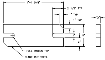
COUNTERWEIGHT DETAIL
