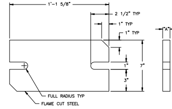
COUNTERWEIGHT DETAIL
