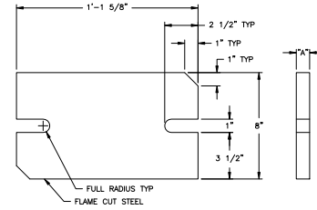
COUNTERWEIGHT DETAIL
