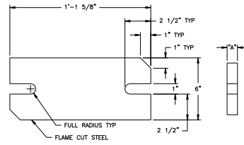
COUNTERWEIGHT DETAIL
