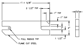
COUNTERWEIGHT DETAIL
