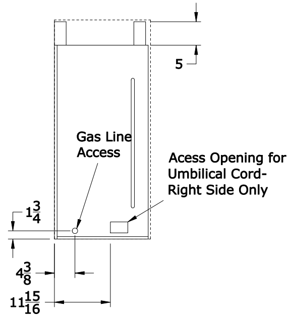
RIGHT SIDE
